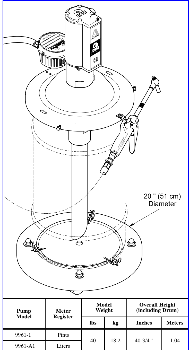
Figure 1 Medium-Pressure Portable Pump Models 9961-1 and 9961-A1
